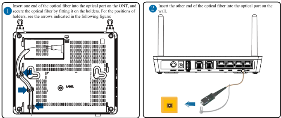
Figure 1-10 Optical ports on the HG8245H
