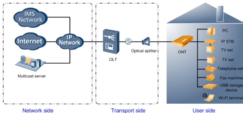
Figure 1-1 Network topology of the ONT
