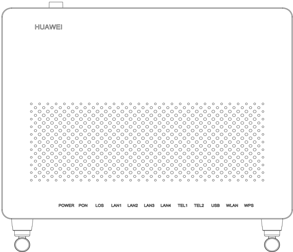
Figure 1-11 LEDs on the HG8245H
