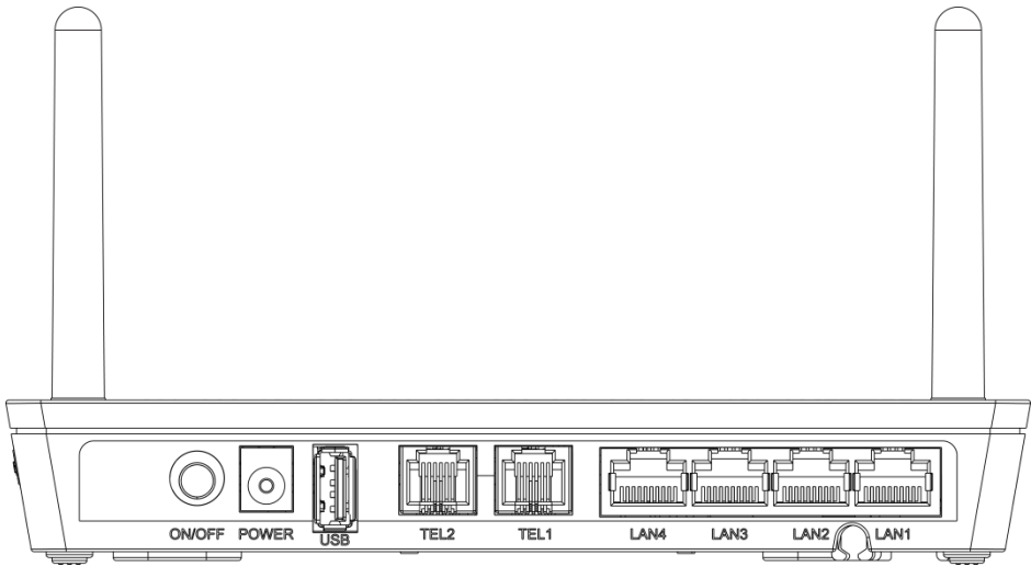
Figure 1-8 Ports and buttons on the rear panel of the HG8245H
