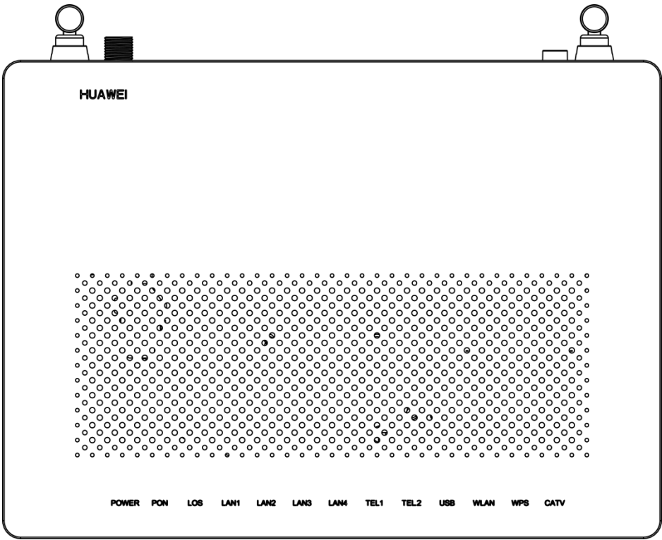
Figure 1-6 LEDs on the HG8247H
