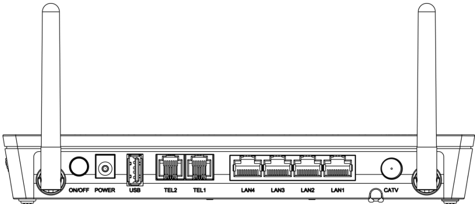
Figure 1-3 Ports and buttons on the rear panel of the HG8247H
